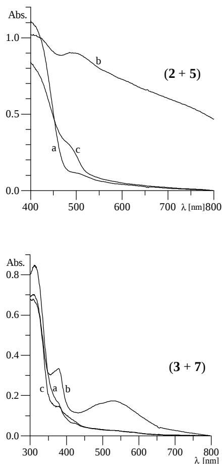
Fig. 5 UV/Vis spectra of the cocrystals of meso -1,2-bis(4-dimethylaminophenyl)-1,2-ethanediol (2) and bis(4-cyanobenzylidene)ethylenediamine (2 + 5) and of 1,2-bis(4-methoxyphenyl)-1,2-ethanediol and bis(4-nitrobenzylidene)ethylenediamine (3 + 7) in diffuse reflection on KBr, before (a) and after (b) irradiation, and after heating (c). For details see text.
