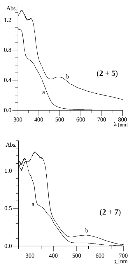
Fig. 6 UV/Vis spectra of cocrystals (2 + 5) and (2 + 7) in KBr matrix, before (a) and after (b) irradiation (molar ratio 1 : 5 × 10 -3 ).
